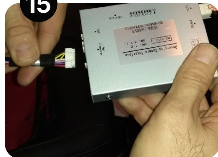
Connect to camera power loom (F)
