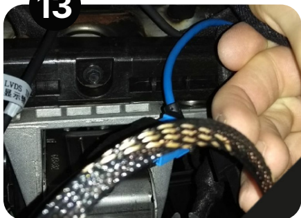
Connect other end of Pass Through into car (D)
